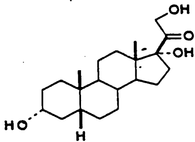
Tetrahydrocortexolone (THS)
